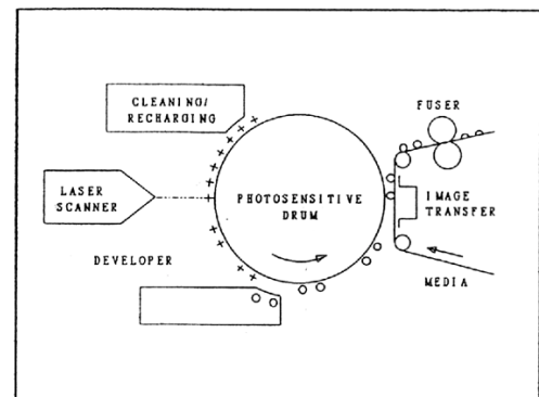
Laser Printing
