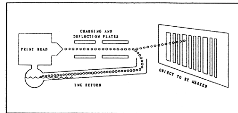
Deflection Ink Jet
